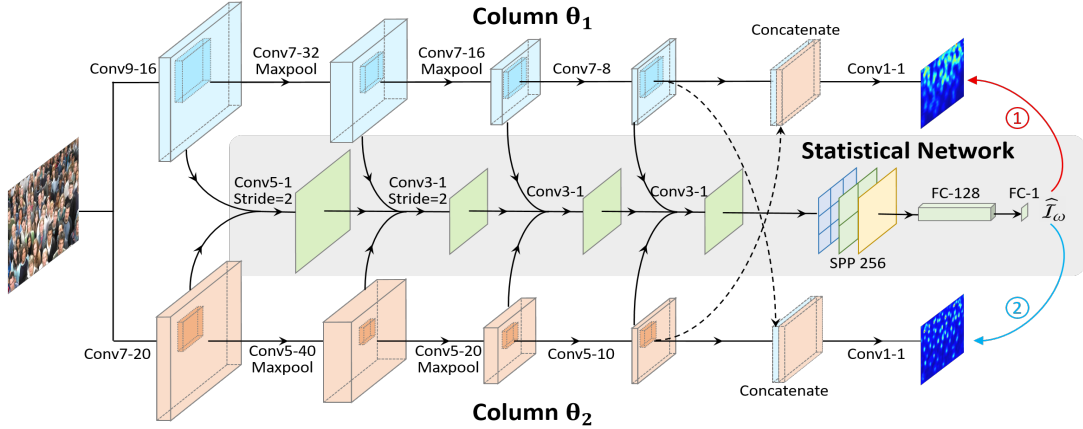
Figure 3: Overview of our Multi-column Mutual Learning (McML) strategy. It is equivalent to adding a statistical network to estimate the mutual information \widehat{I}_\omega between columns. By minimizing the mutual information, it can guide multi-columns to learn different scale information. Additionally, McML is a mutual learning scheme as arrows ① and ②, where each column is alternately optimized while keeping the other columns fixed on each mini-batch training data. Specifically, this is an example of two columns ( \Theta_1 and \Theta_2 ) in MCNN [69]. ConvX-Y implies a convolutional layer has Y filters with X×X kernel size. The stride of all convolutional layers is 1, except for the special reminder. MaxPool is the max pooling layer with a stride of 2. [Best viewed in color].
