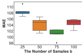
Figure 4: Effects of samples b . Table 5: The values of \alpha .
